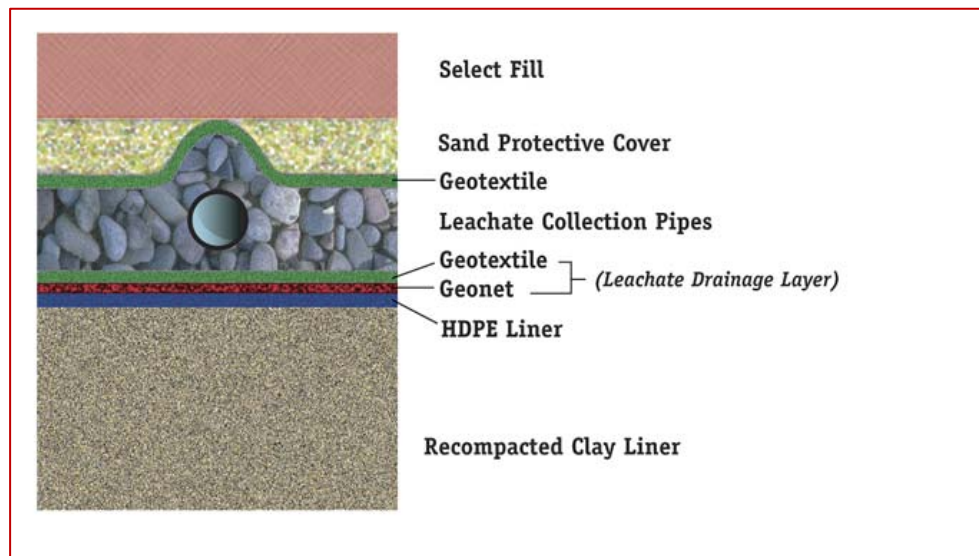
Typical Cross Section at Landfill Site
