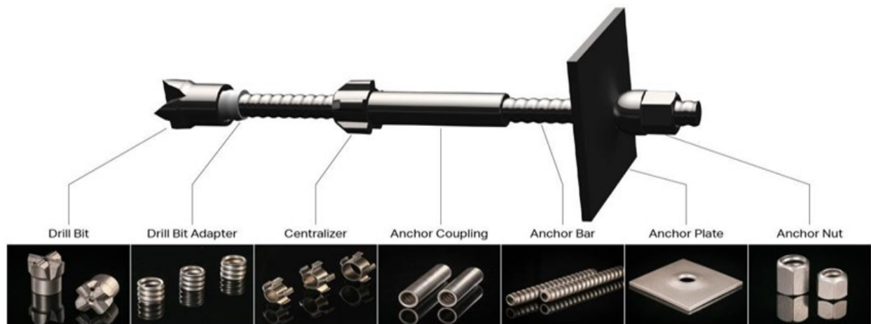
Fig1: Self drilling anchors with accessories
