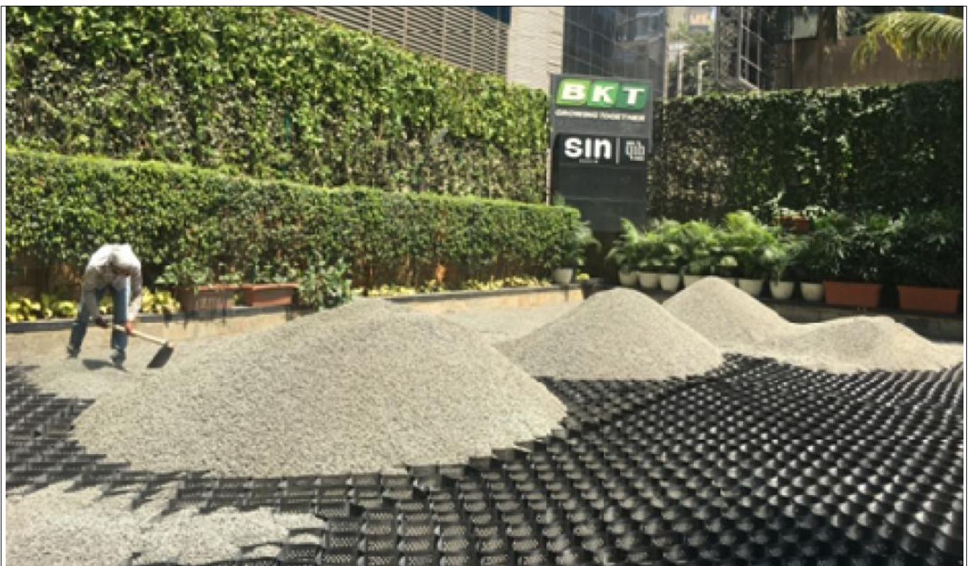
Filling of Geocell with Crushed stone / Grit
