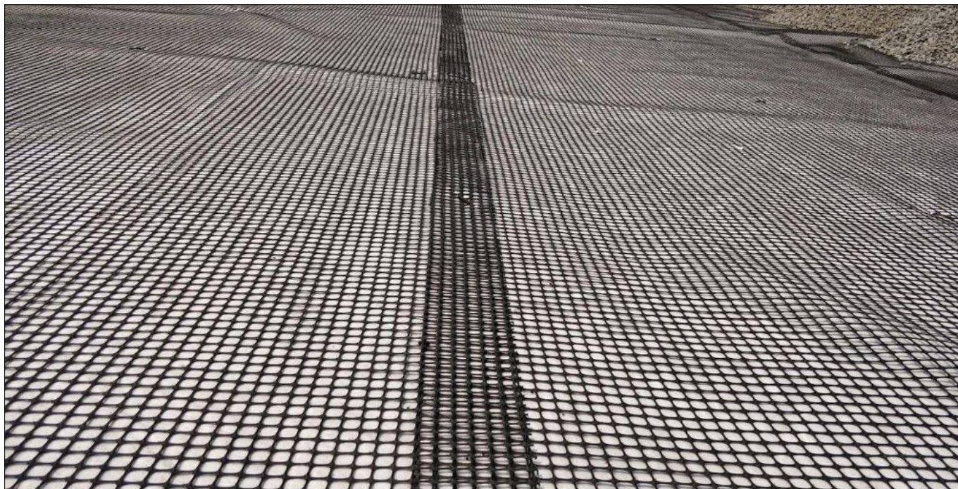
Geogrid Overlaps of 150mm at the side edges
