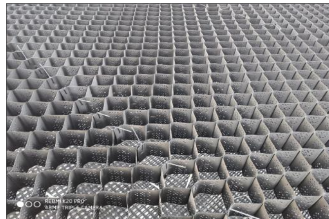
Photo 6 - Laying of Techcell Geocell over TechGrid Geogrid
